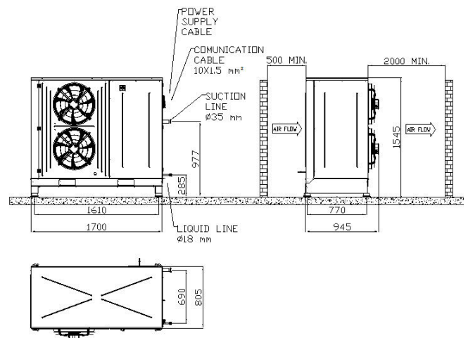
REMOTE CONDENSING UNIT
